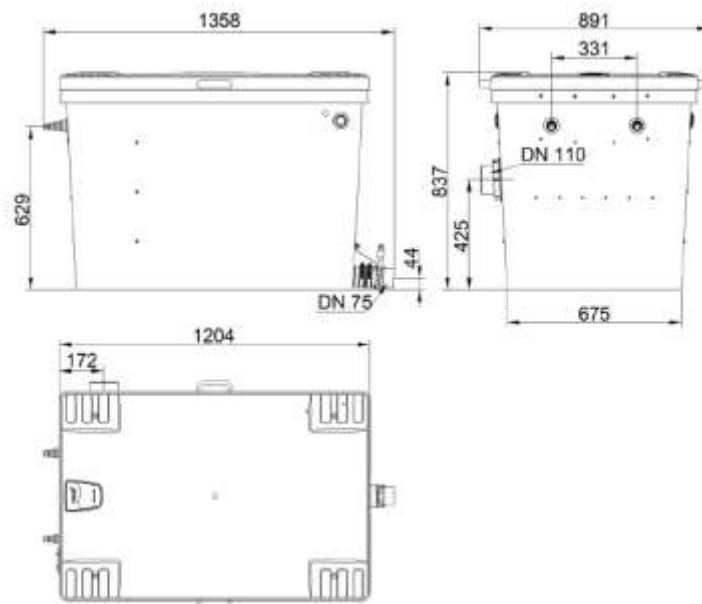
BioTec ScreenMatic 1 145000
