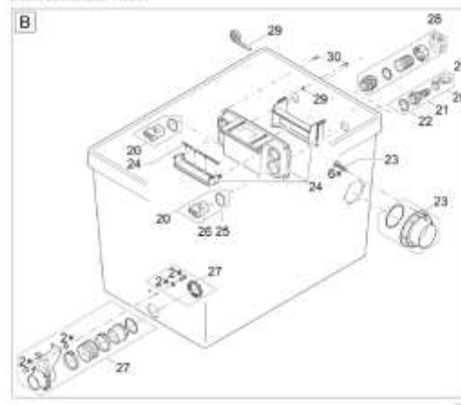
BioTec ScreenMatic 1 145000
