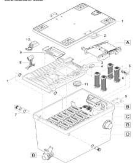
BioTec ScreenMatic 1 145000
